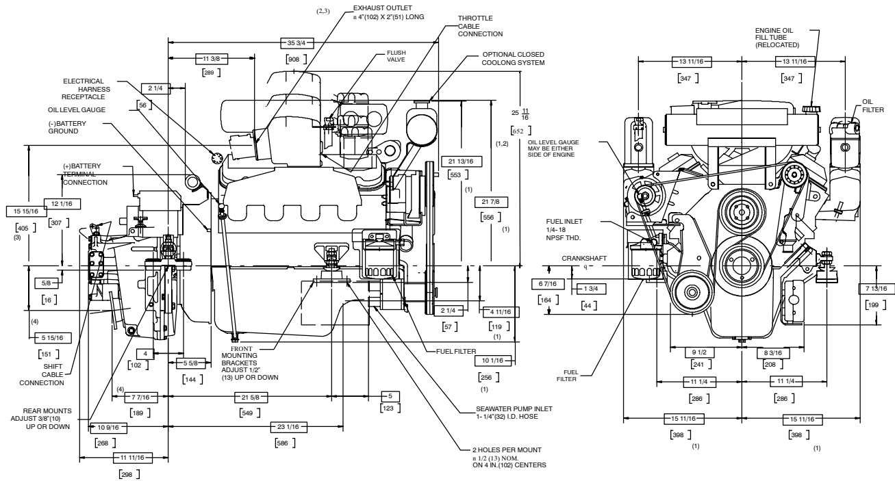
MIE 454 MAGNUM MPI HORIZON WITH VELVET DRIVE 5000A) DOWN-ANGLE TRANSMISSION
