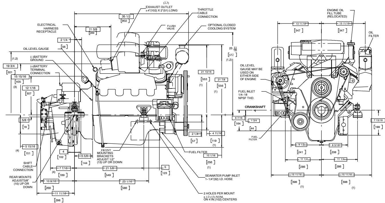
MIE 8.2L MPI BLUEWATER WITH (VELVET DRIVE 5000A) DOWN-ANGLE TRANSMISSION
